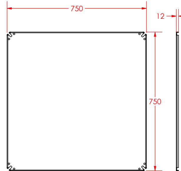
MOUNTING PLATE
