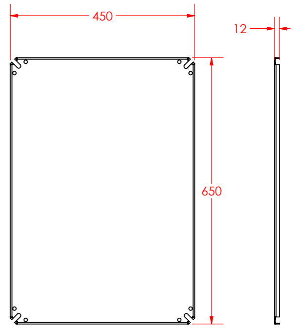
MOUNTING PLATE
