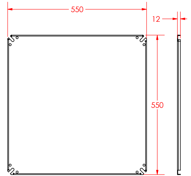
MOUNTING PLATE
