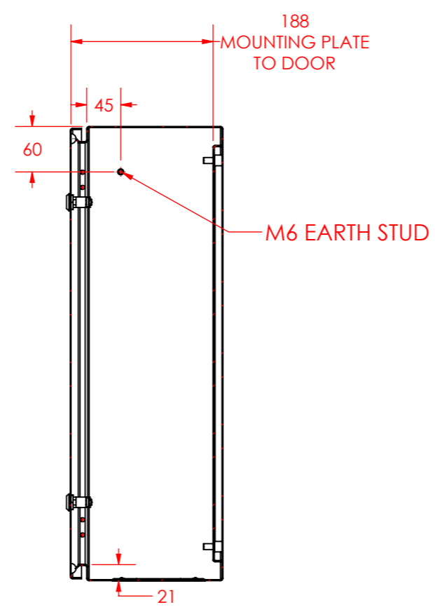
SECTION A-A SCALE 1:7
