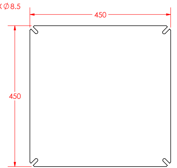
MOUNTING PLATE
