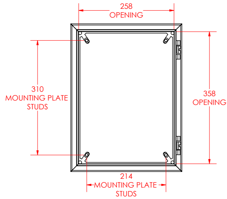
FRONT VIEW WITHOUT DOOR
