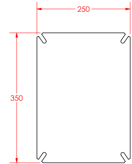
MOUNTING PLATE
