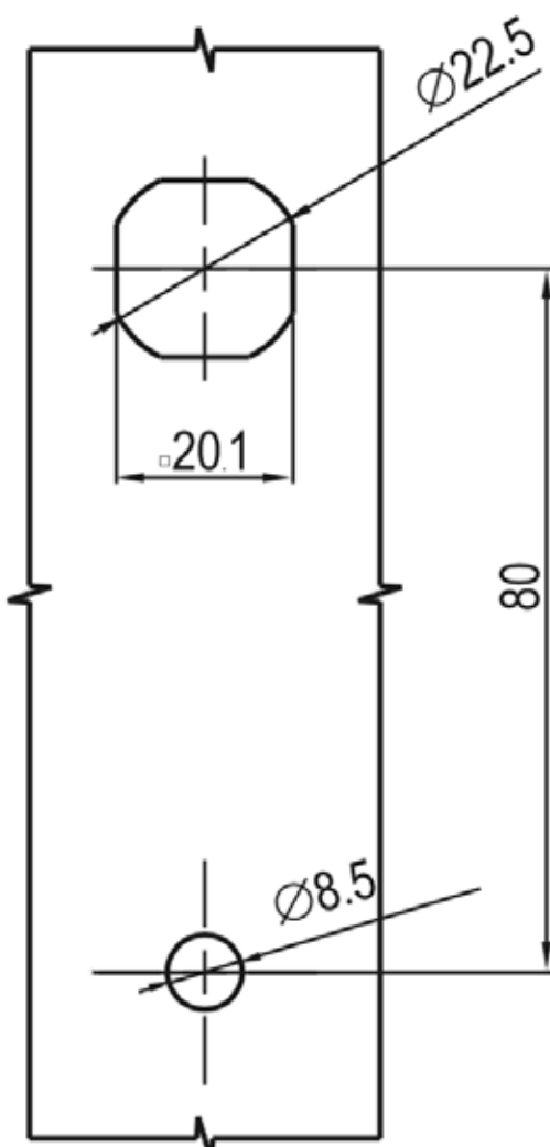
Panel cutou
