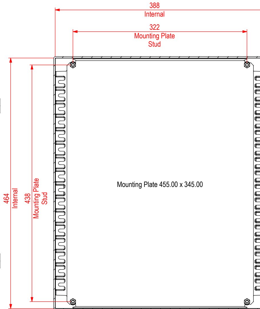
SECTION B-B
